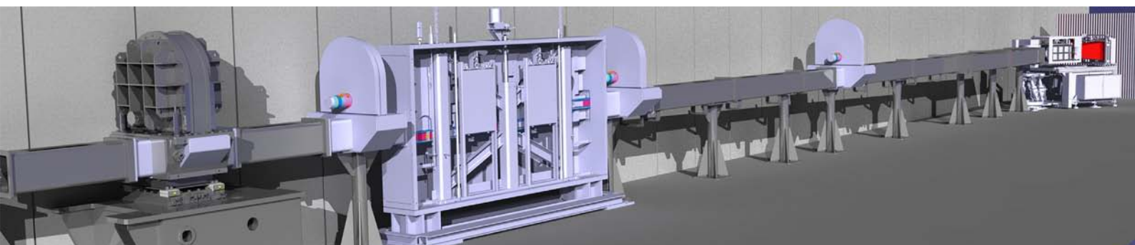
Fig. 4: Impression of the reflectometer outline showing the elliptic guide section with chopper 1 (left) and polarizer changing section ending with the sample and detector stages (right).
