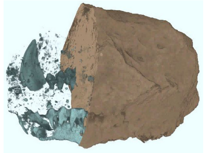
An upper jaw entirely embedded in a block of limestone found in South Africa, possible of an ape, like a baboon. In the neutron tomography data-set, the surrounding limestone is set to invisible so the jaw bones and teeth become visible, along with several pebbles.
